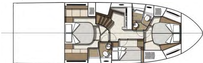
3 cabin layout
